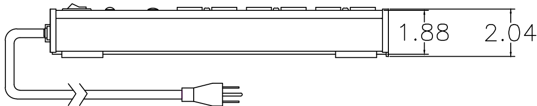
SIDE VIEW
