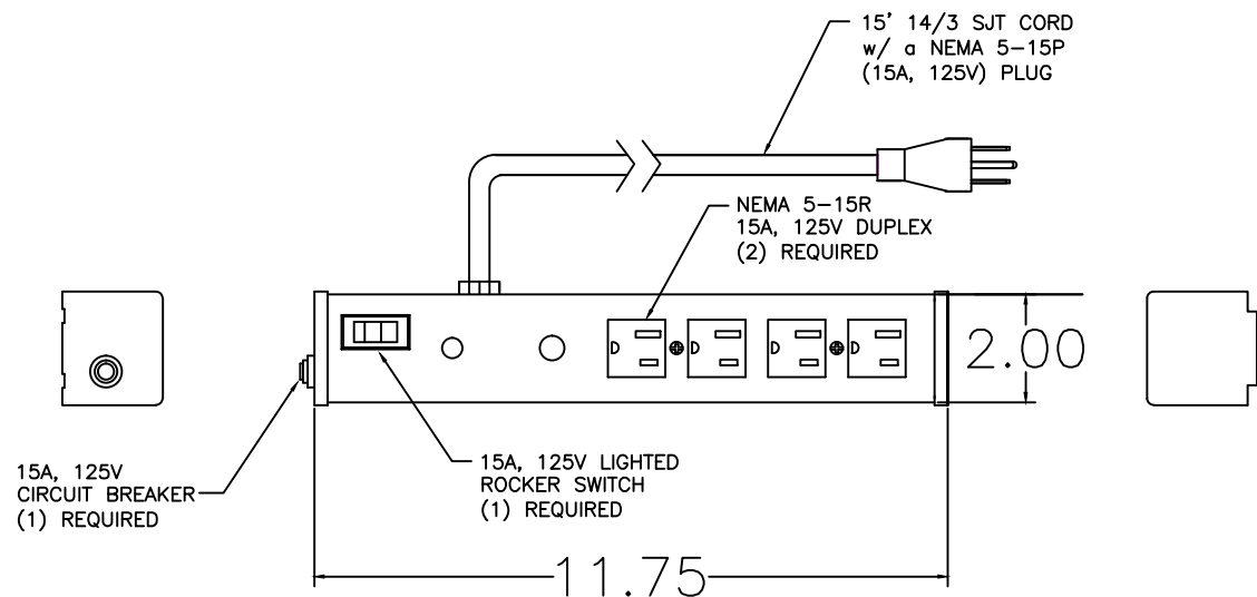
FRONT VIEW
